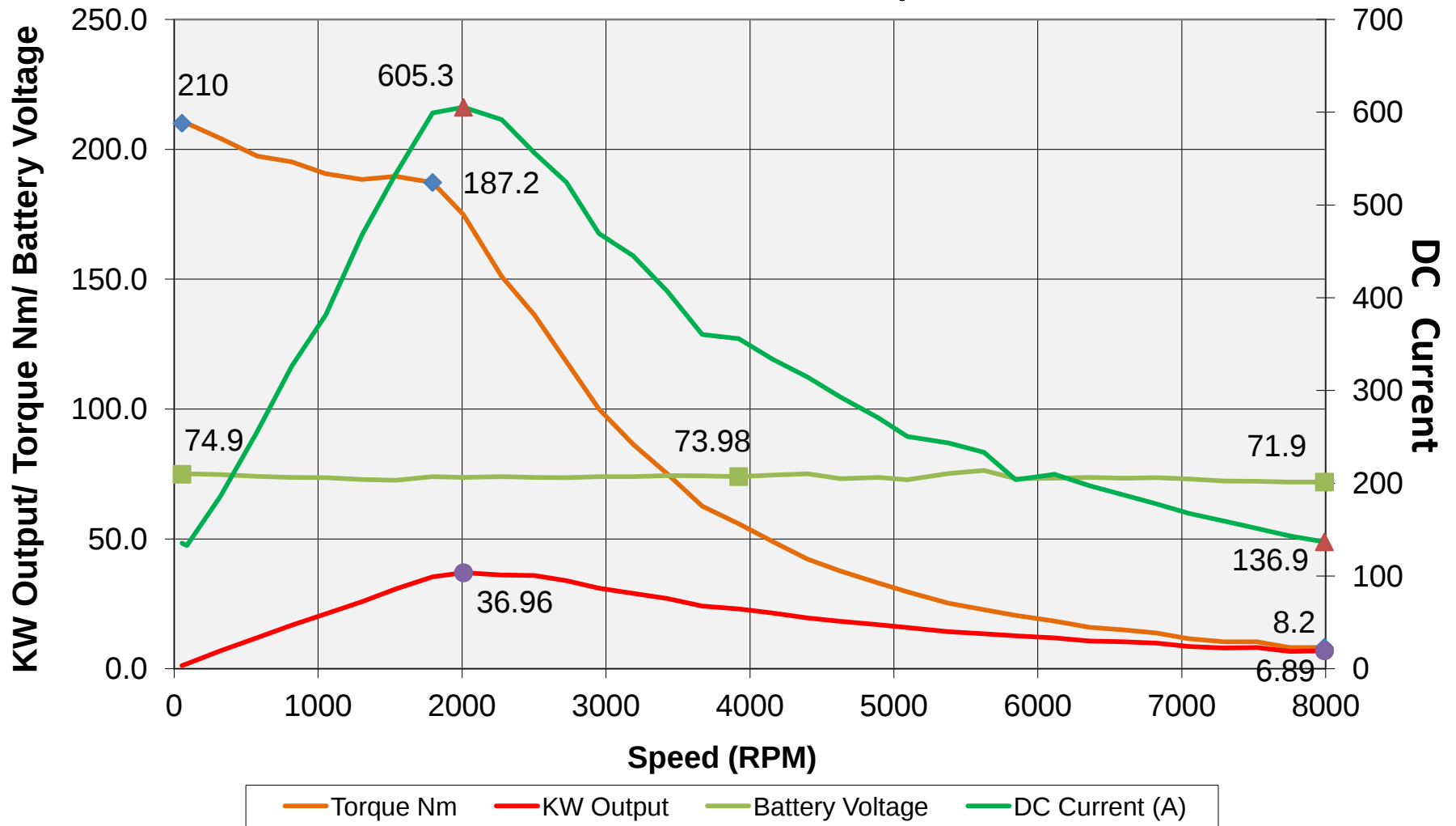
HPEVS AC-51 Metric Peak Graph 72 Volts/650 Amps
