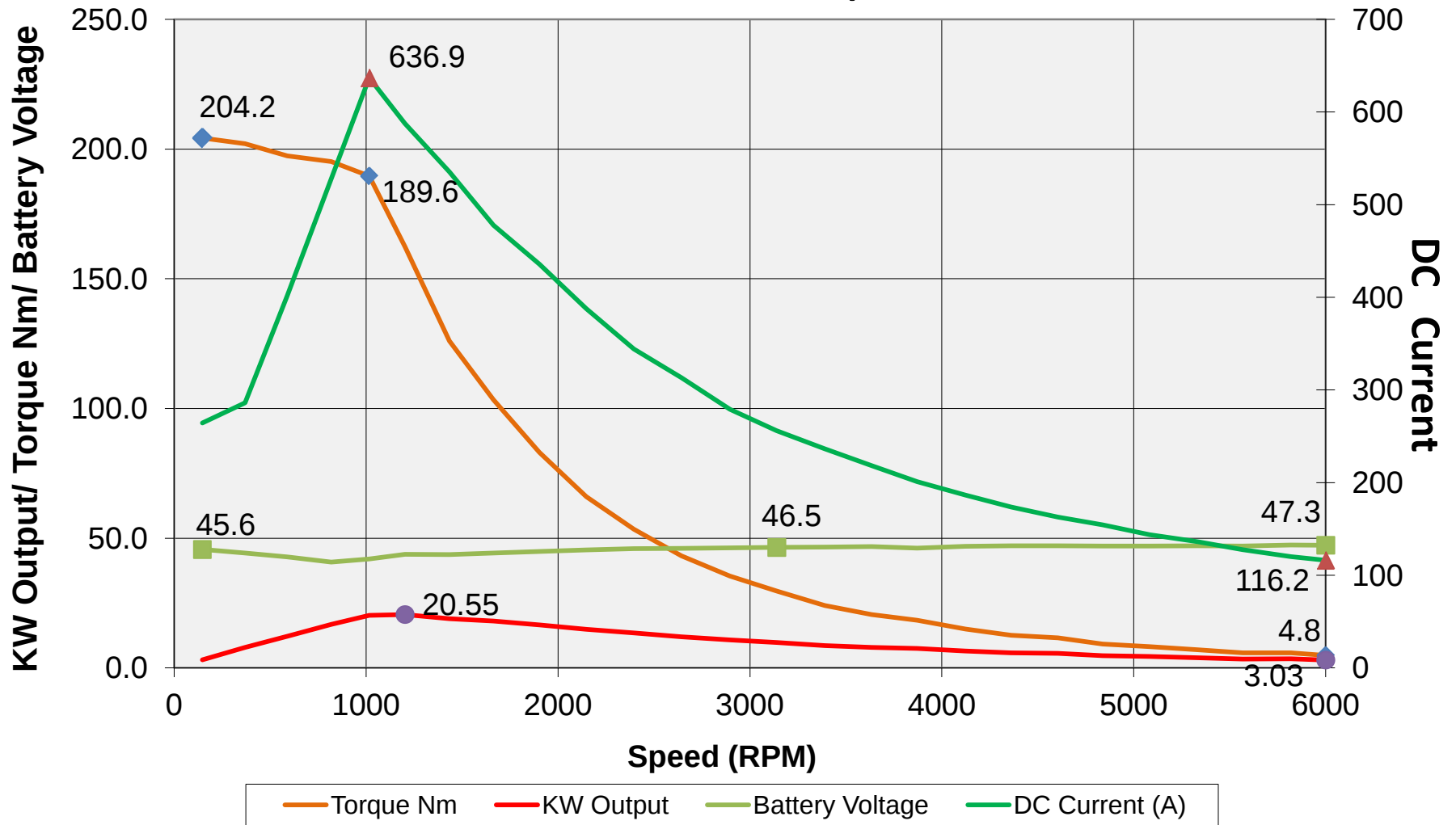
HPEVS AC- Metric Peak Graph Volts/ Amps
