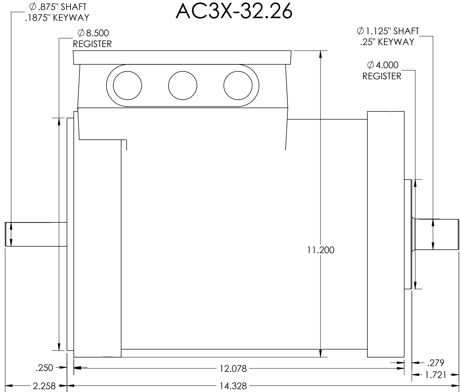
SIDE VIEW
