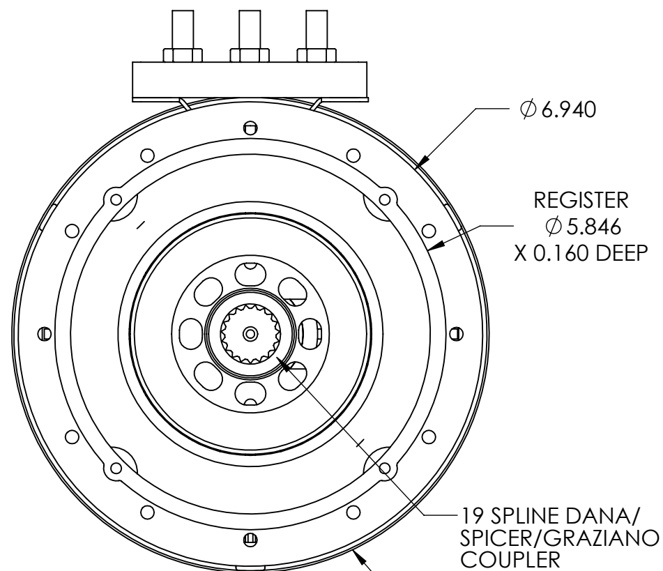
DRIVE END
