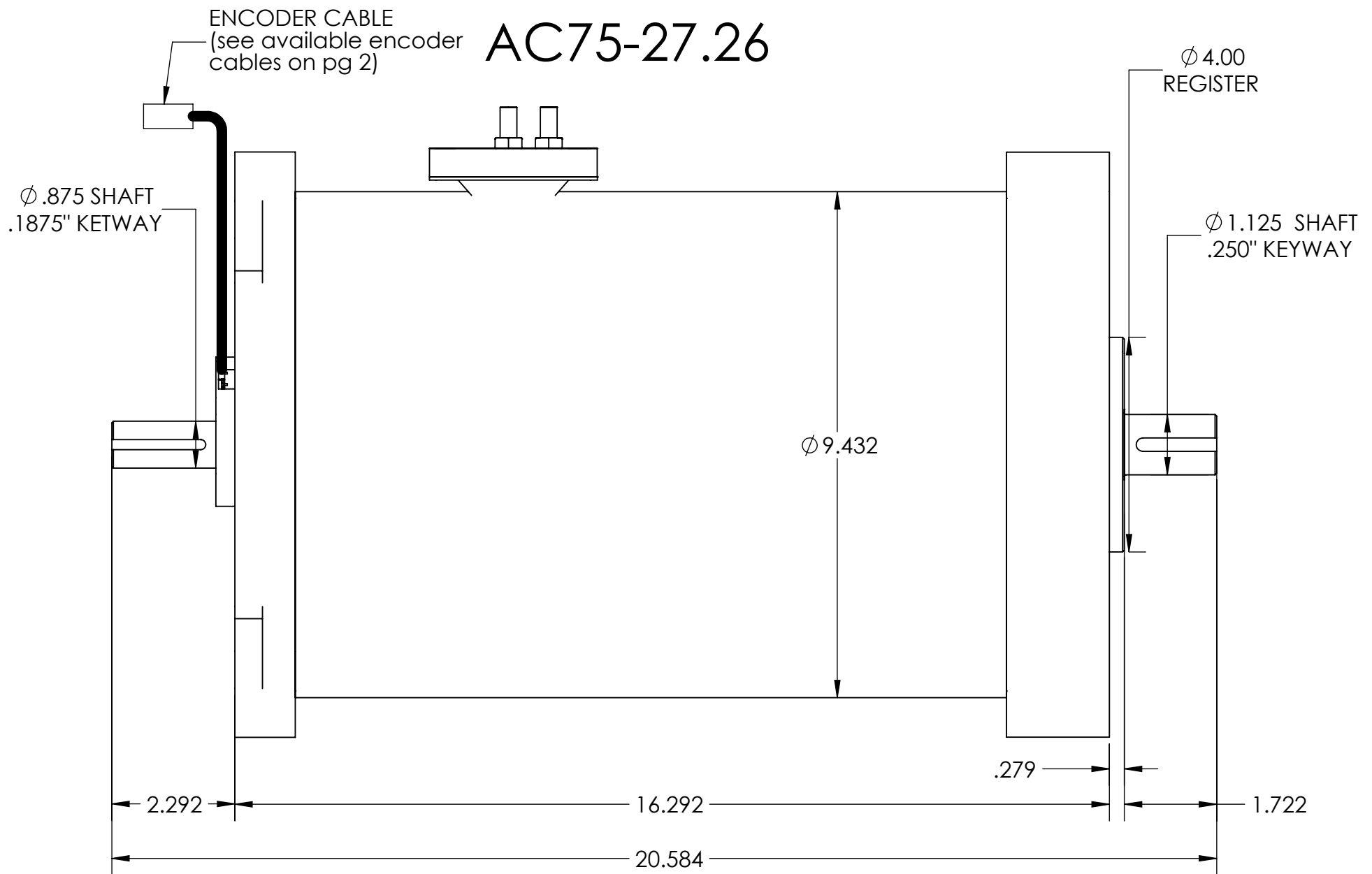
SIDE VIEW
