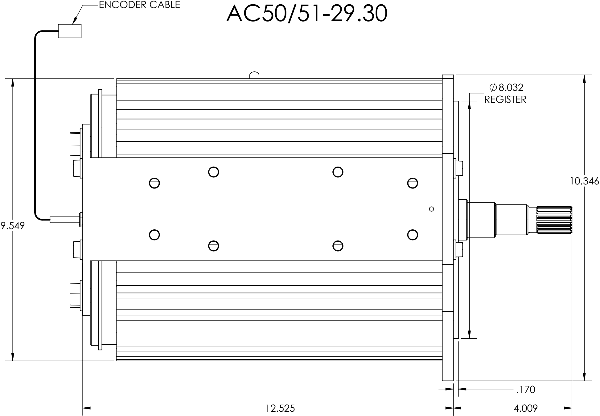
SIDE VIEW
