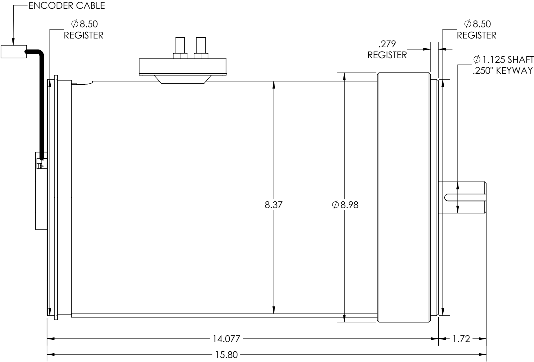
SIDE VIEW
