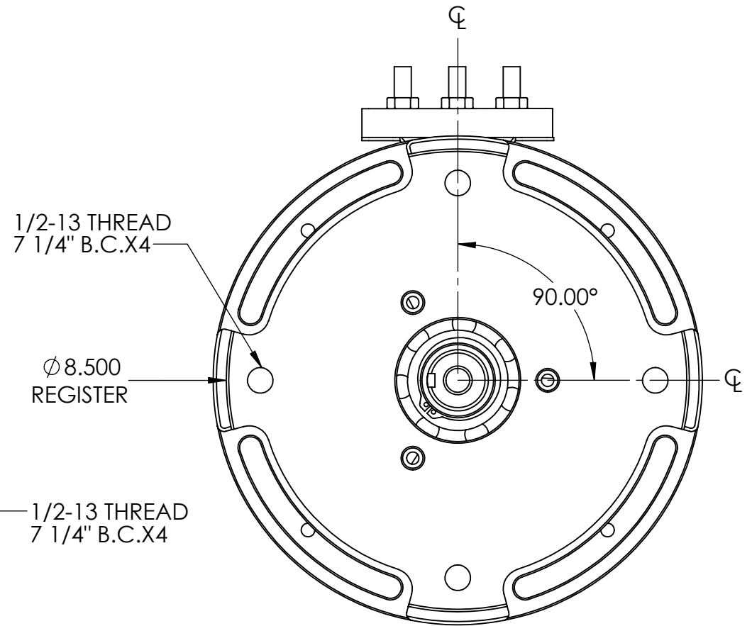
DRIVE END
