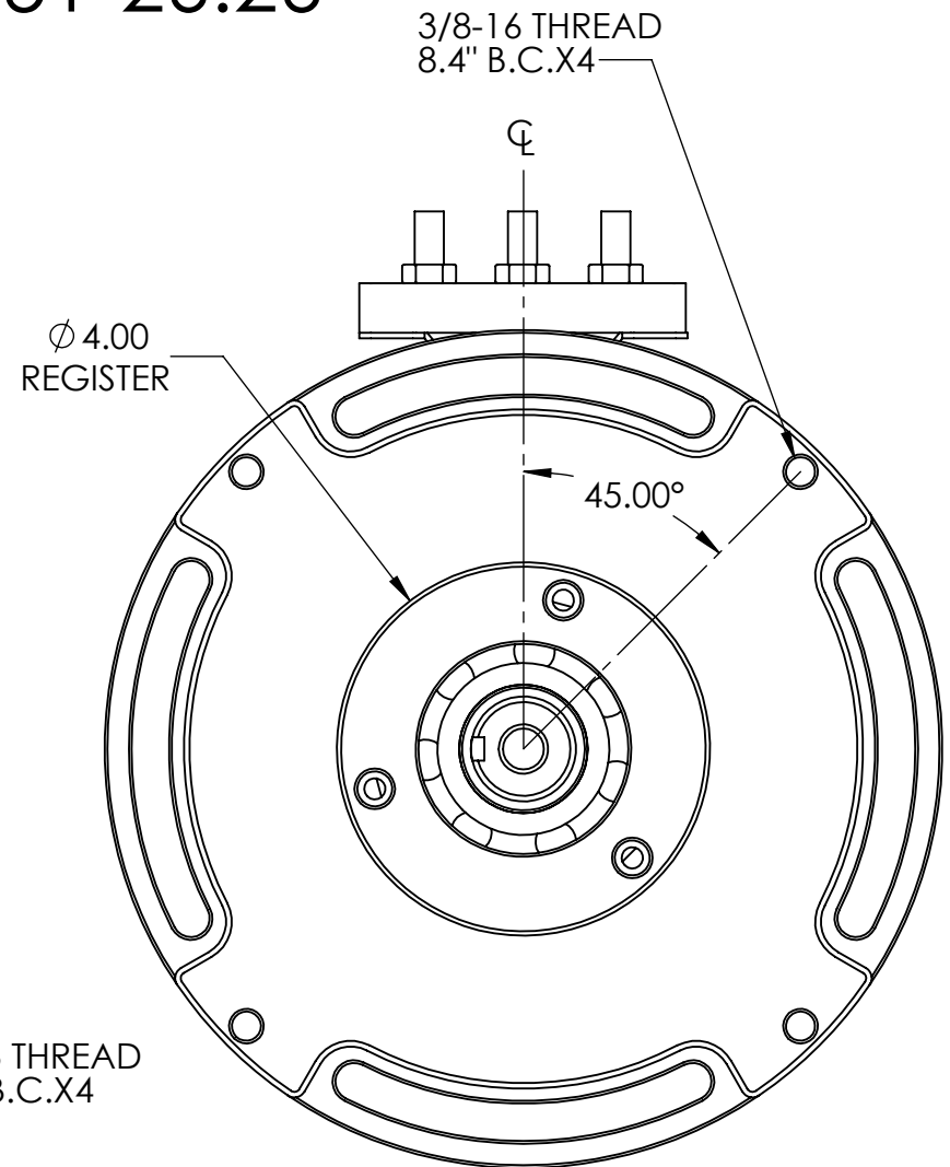
DRIVE END
