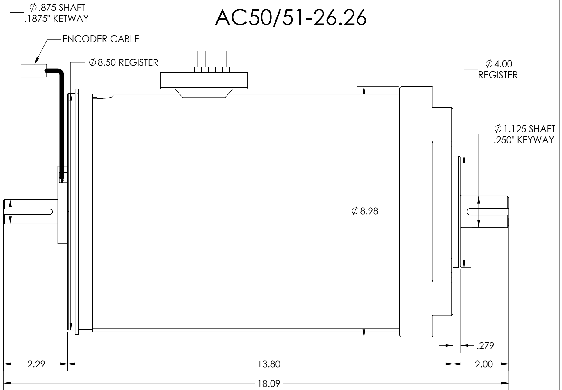
SIDE VIEW
