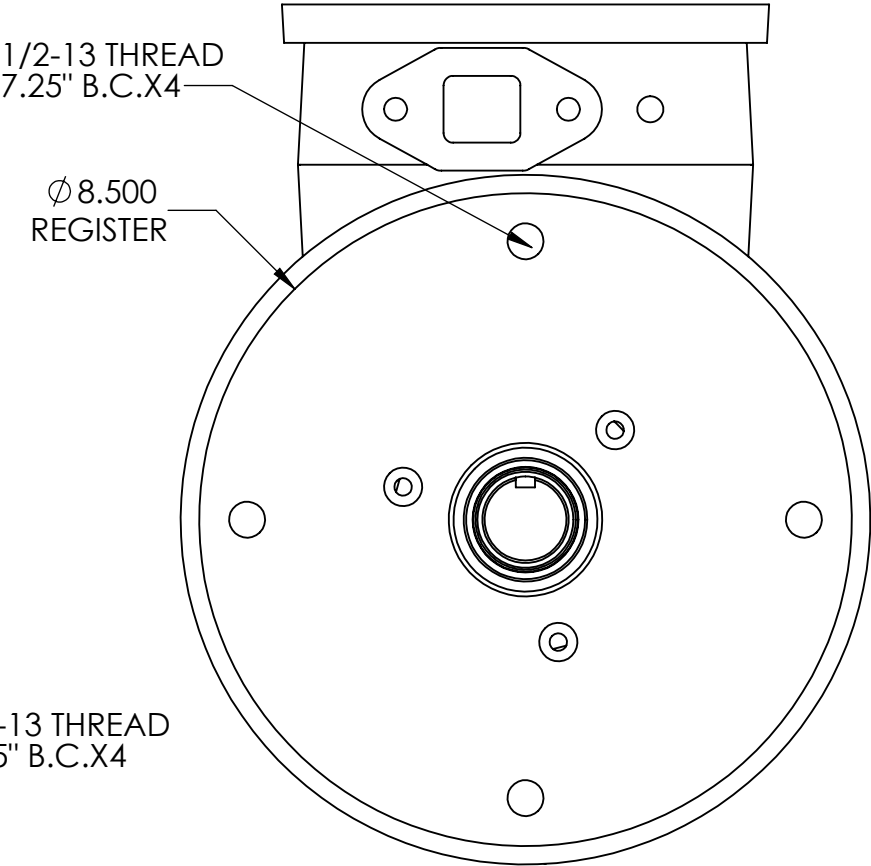
DRIVE END
