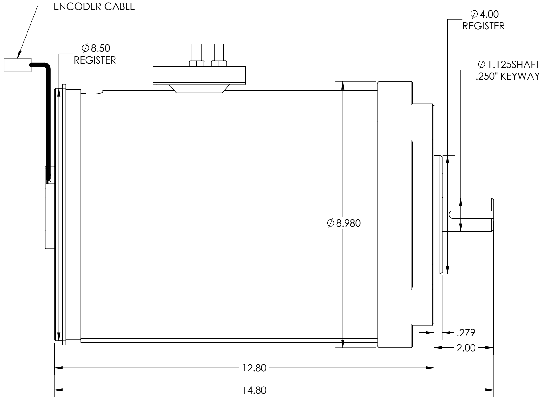
SIDE VIEW
