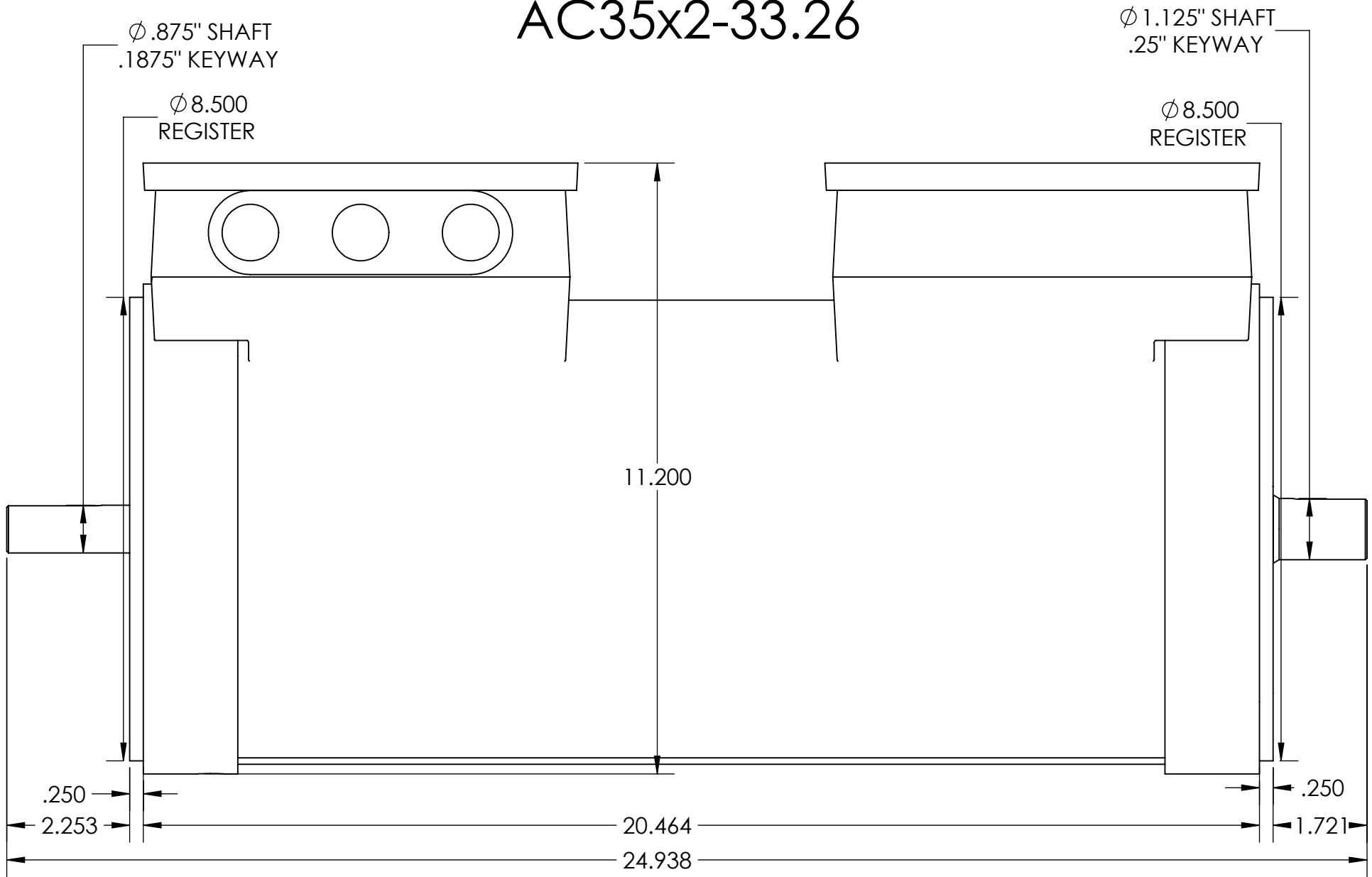
SIDE VIEW
