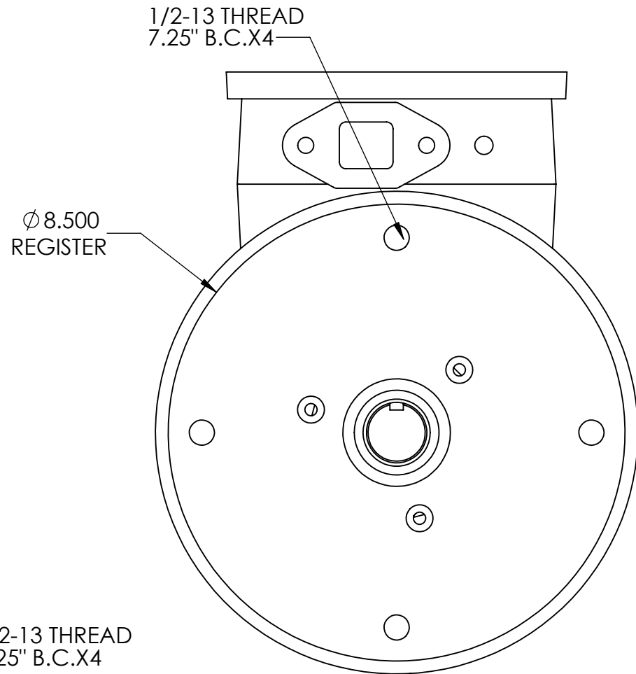
DRIVE END
