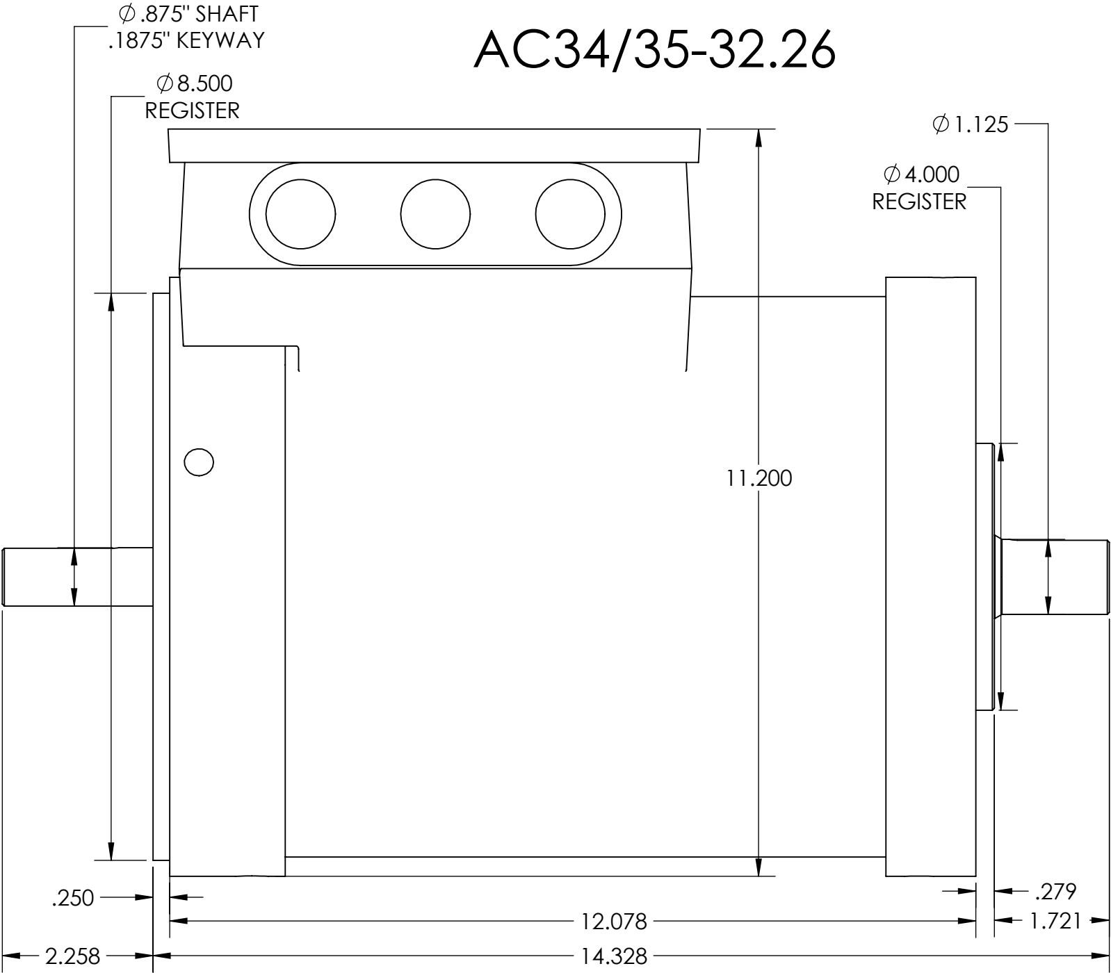
SIDE VIEW
