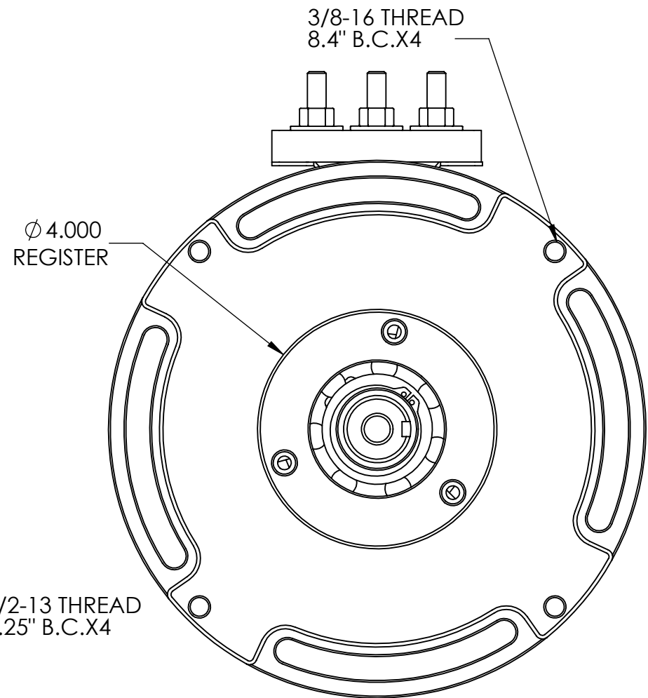
DRIVE END
