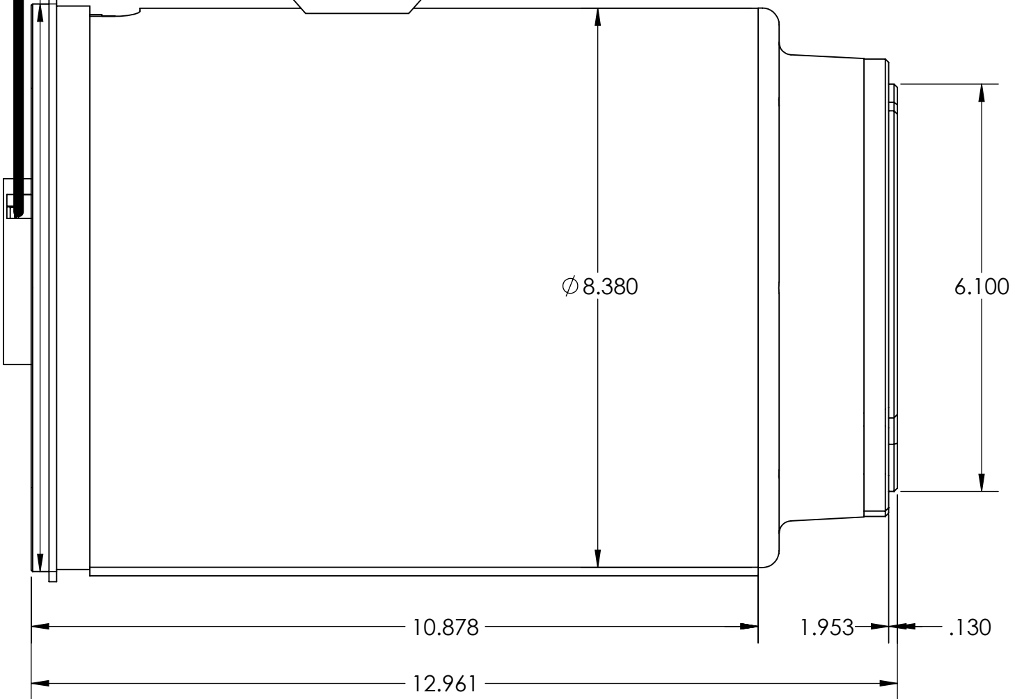
SIDE VIEW
