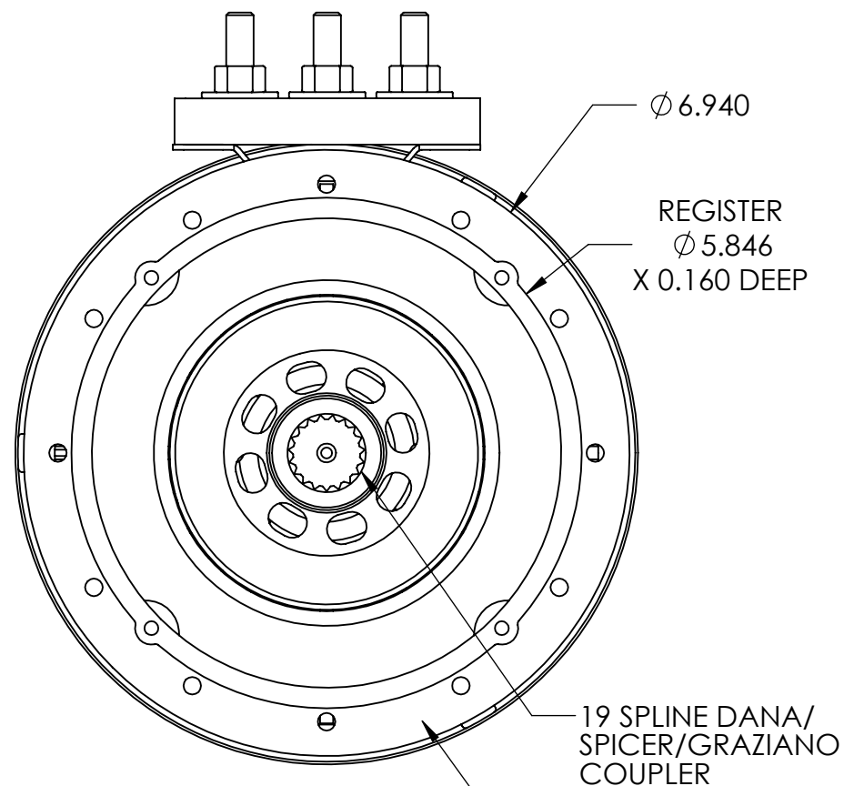
DRIVE END
