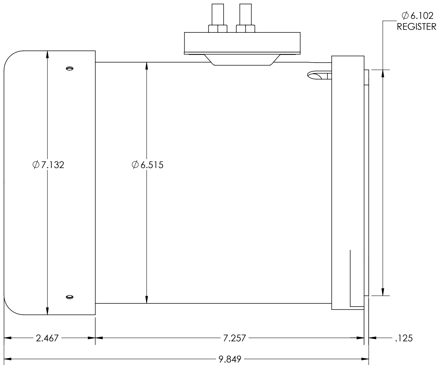
SIDE VIEW
