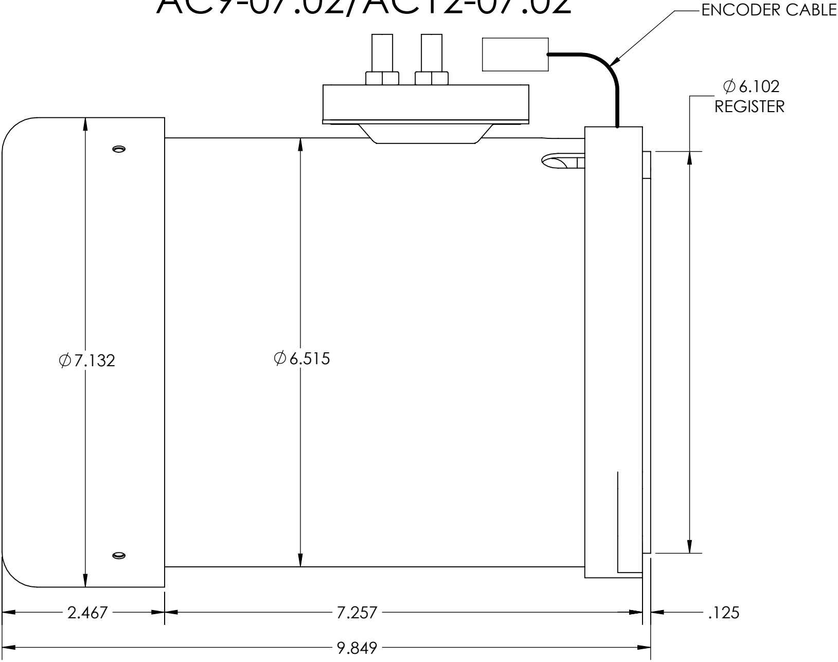
SIDE VIEW
