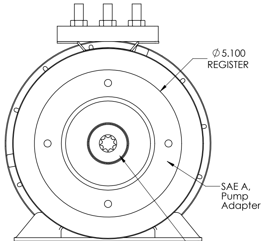
DRIVE END
