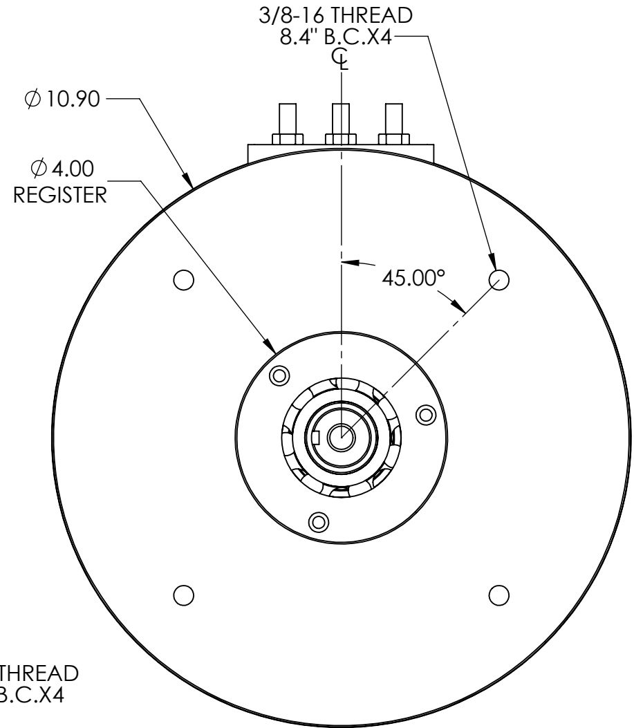
DRIVE END
