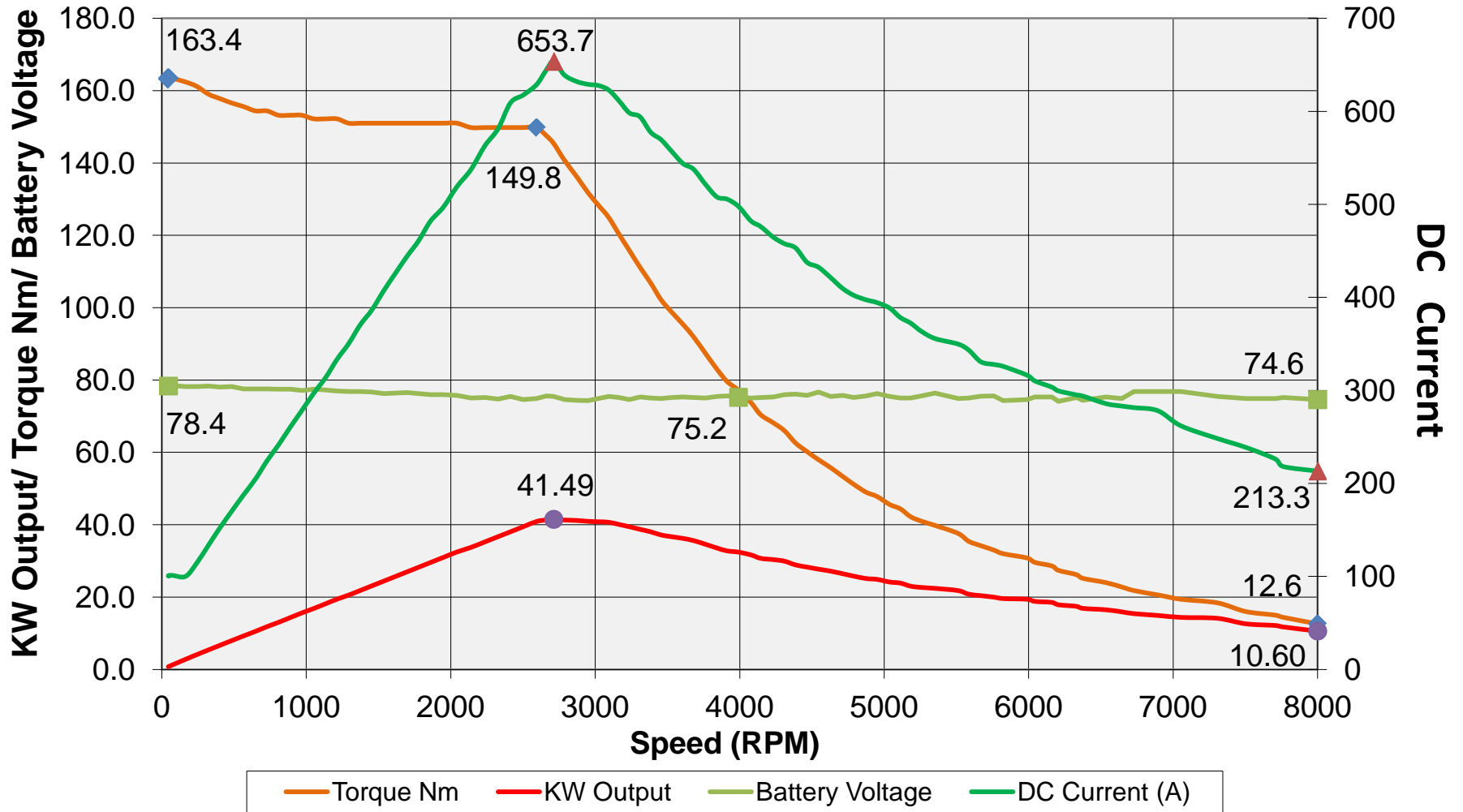
HPEVS AC-50 Metric Peak Graph 72 Volts/650 Amps
